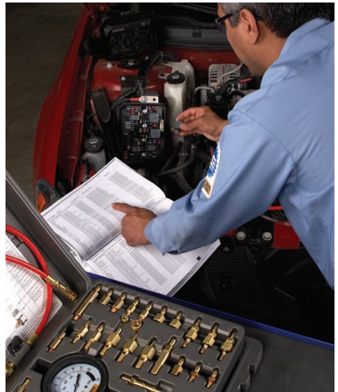
Fuel pump disabling location & procedure
