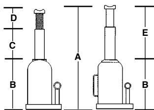
Bottle Jack Dimensions
